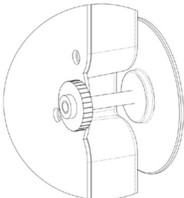
fig 10. Nut should be flush with head of integrated thread in order to allow adequate grip in front facing orientation
